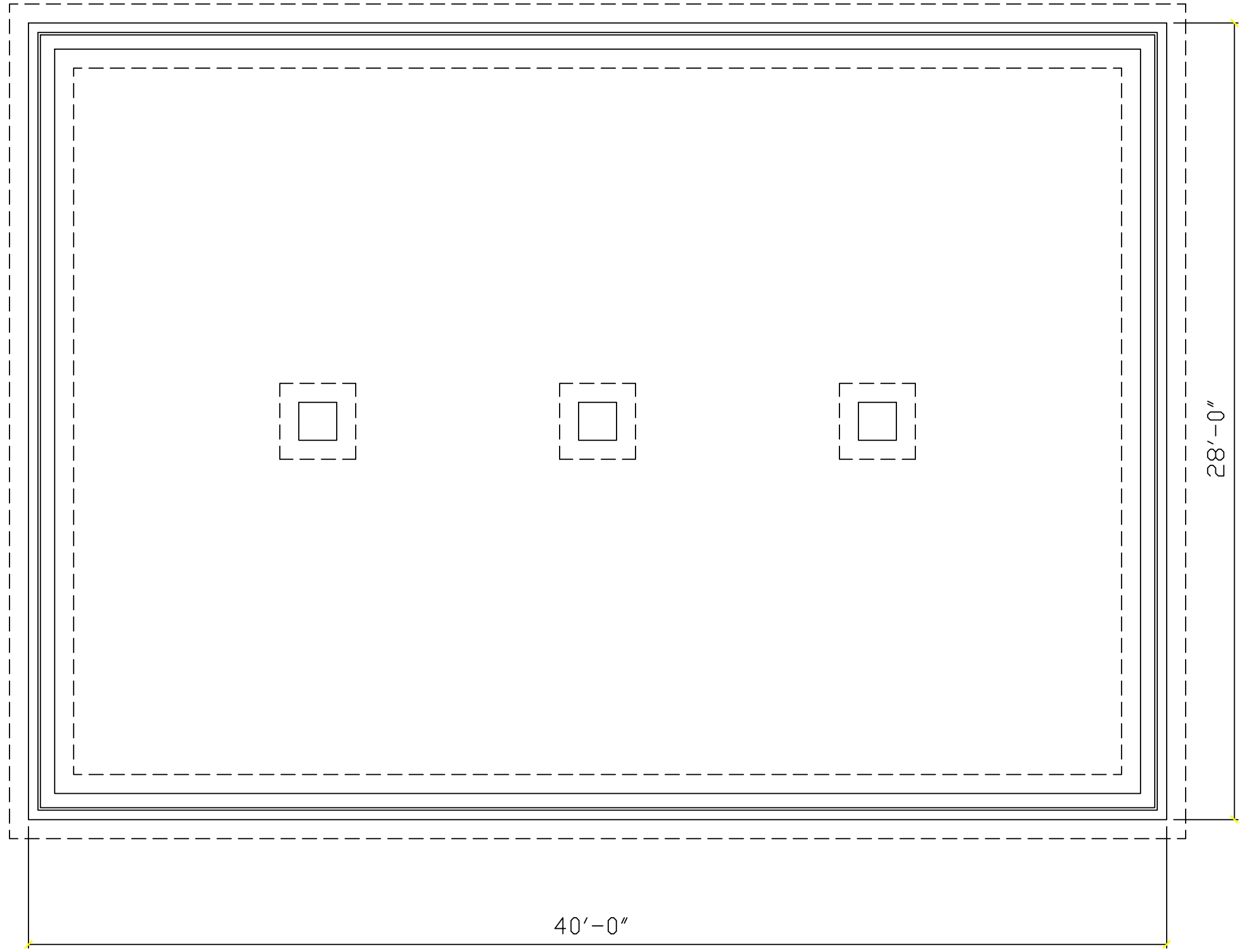
FOUNDATION PLAN
